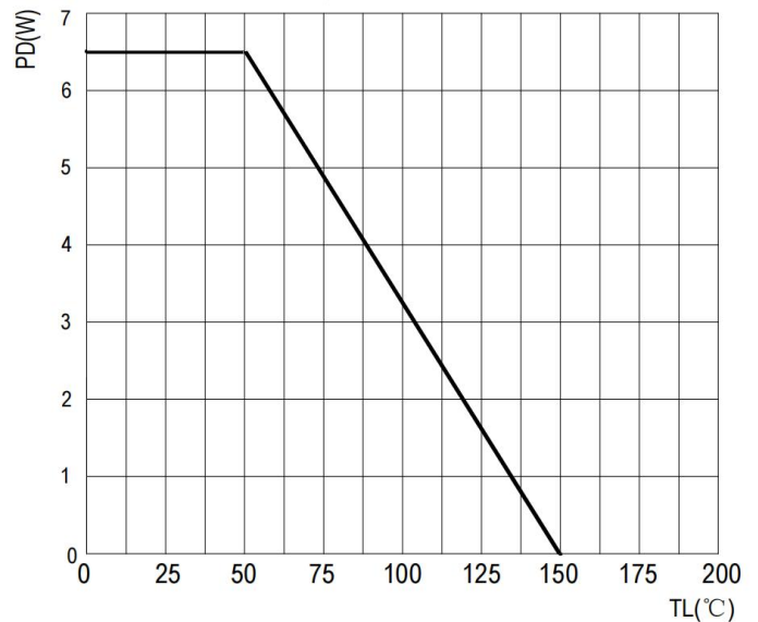
FIG6: Steady State Power Dissipation
