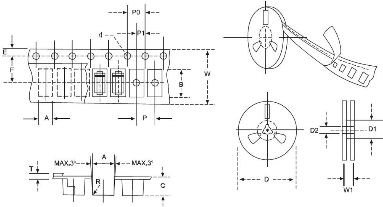
FIG: CONFIGURATION OF SURFACE MOUNTED DEVICES TAPING
