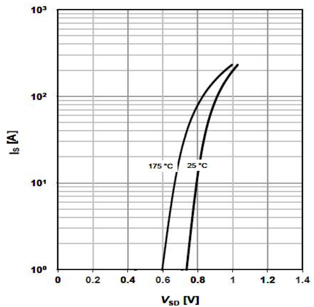
IS -- VSD
